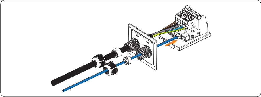
Figure 6-30 Connect the communication cable to Network port
