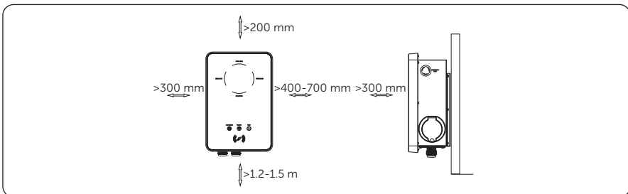
Figure 4-2 Clearance requirement
