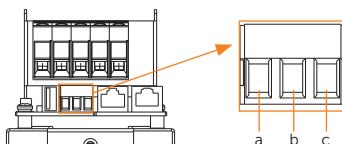
Figure 6-22 RS485 port
