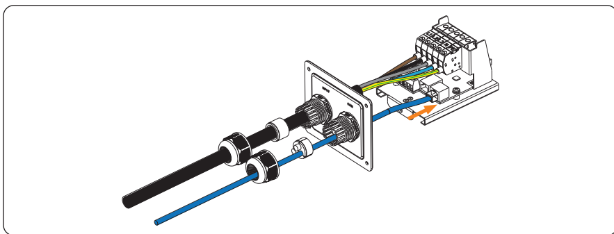
Figure 6-23 Connect the communication cable to RJ45 port
